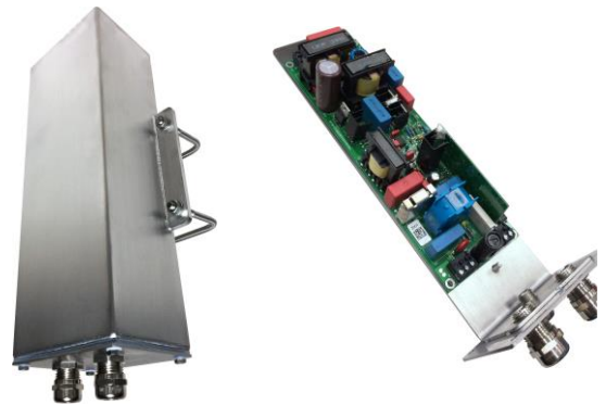
Optional: Industrial ballast in robust stainless steel housing with venting diaphragm (IP 67)
